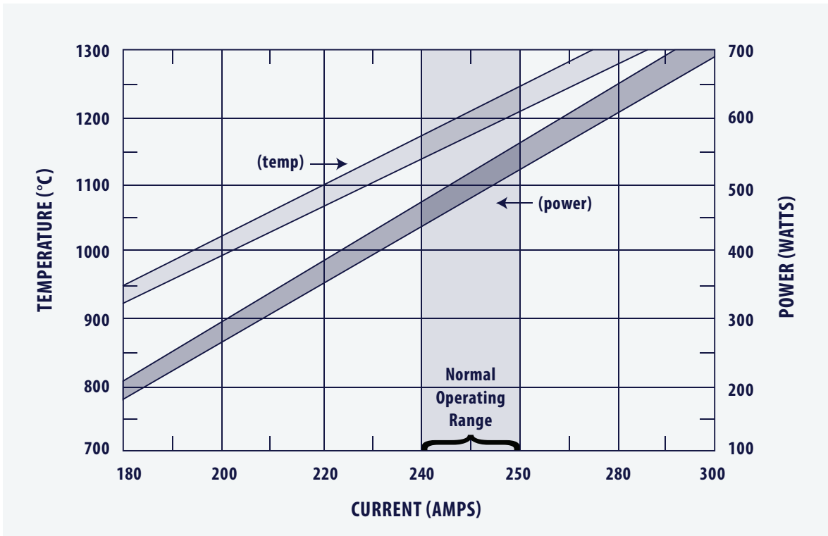
Typical Operating Characteristics of an SO-10 Source
